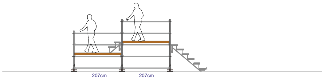
SIDE VIEW
